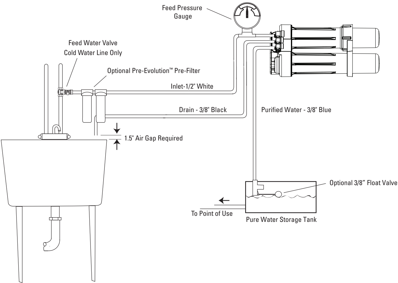
Typical Light Commercial Installation with Storage Tank
